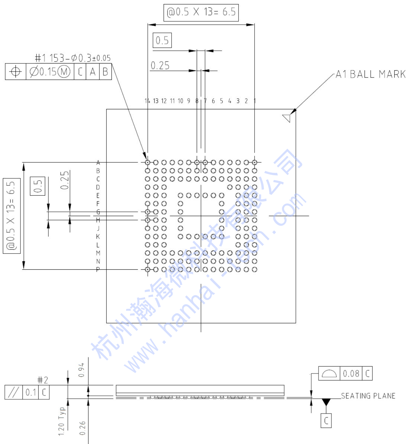
Figure 5 – 11.5 x 13.0 x 1.2mm Bottom & side View
