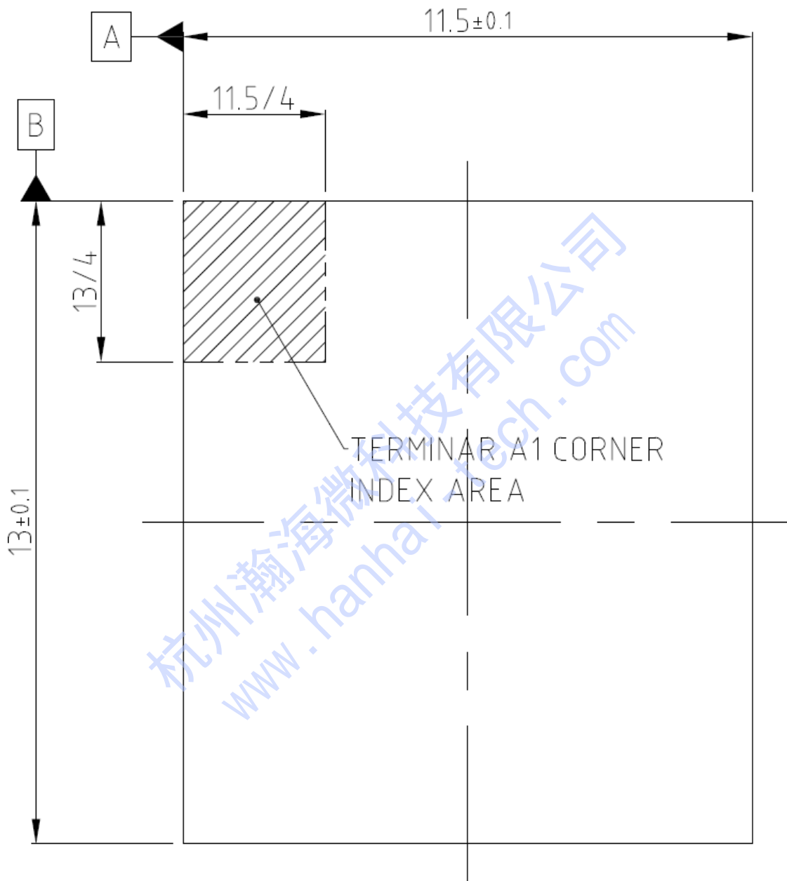
Figure 4 – 11.5 x 13.0 x 1.2mm Top View
