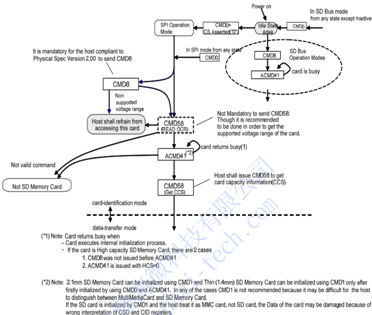
Card State Diagram (SPI mode)
