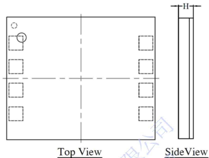
Figure 2: Top View and Side View
