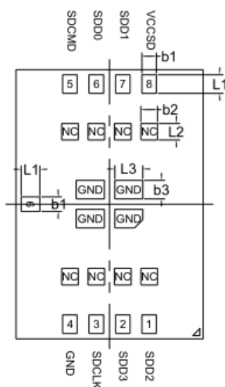
Bottom View
